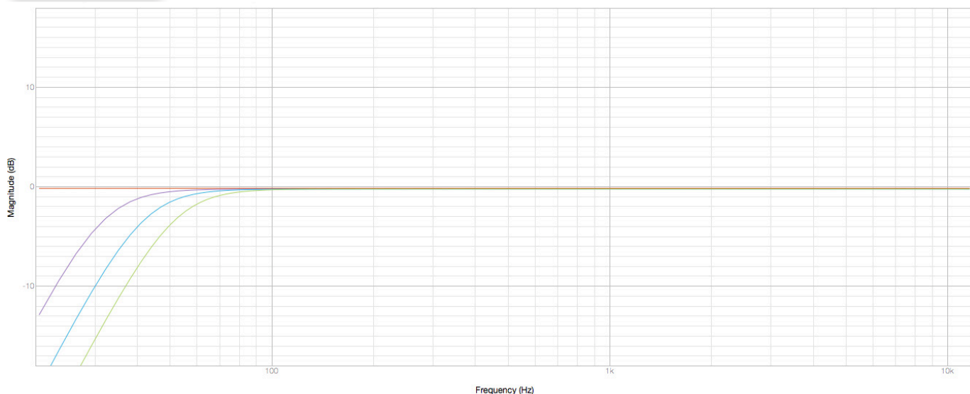
HPF Plots - OFF, 30Hz, 40Hz, 50Hz.
